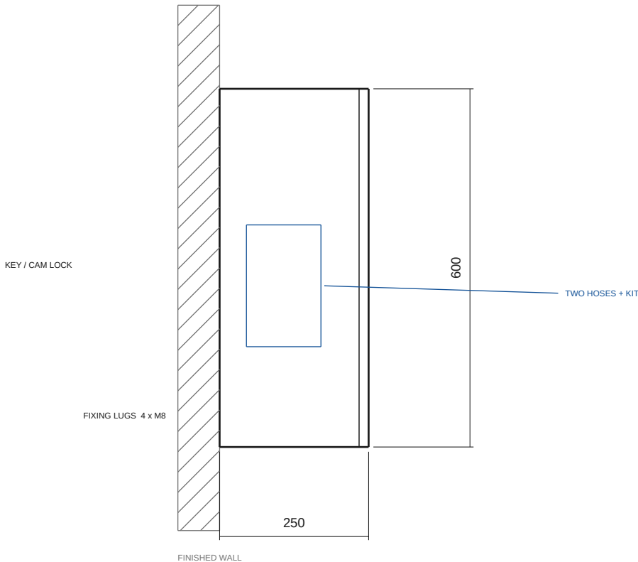
SIDE SECTION
