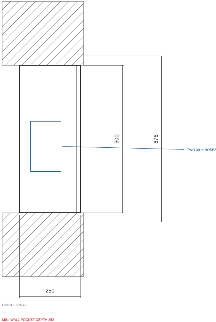
SIDE SECTION
