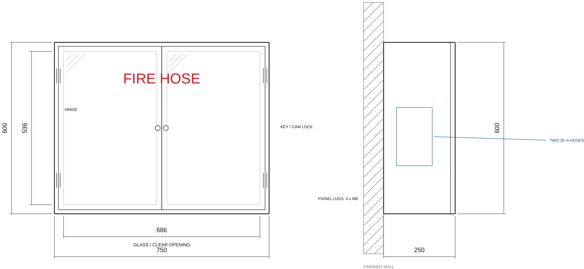
FRONT ELEVATION
