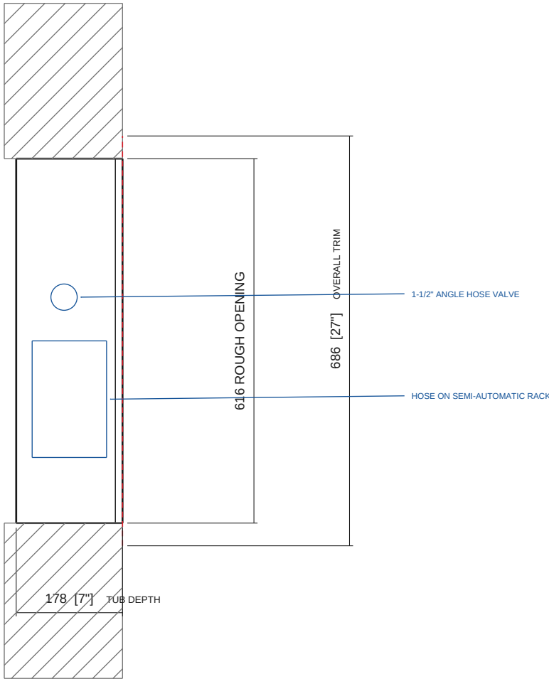
SIDE SECTION
