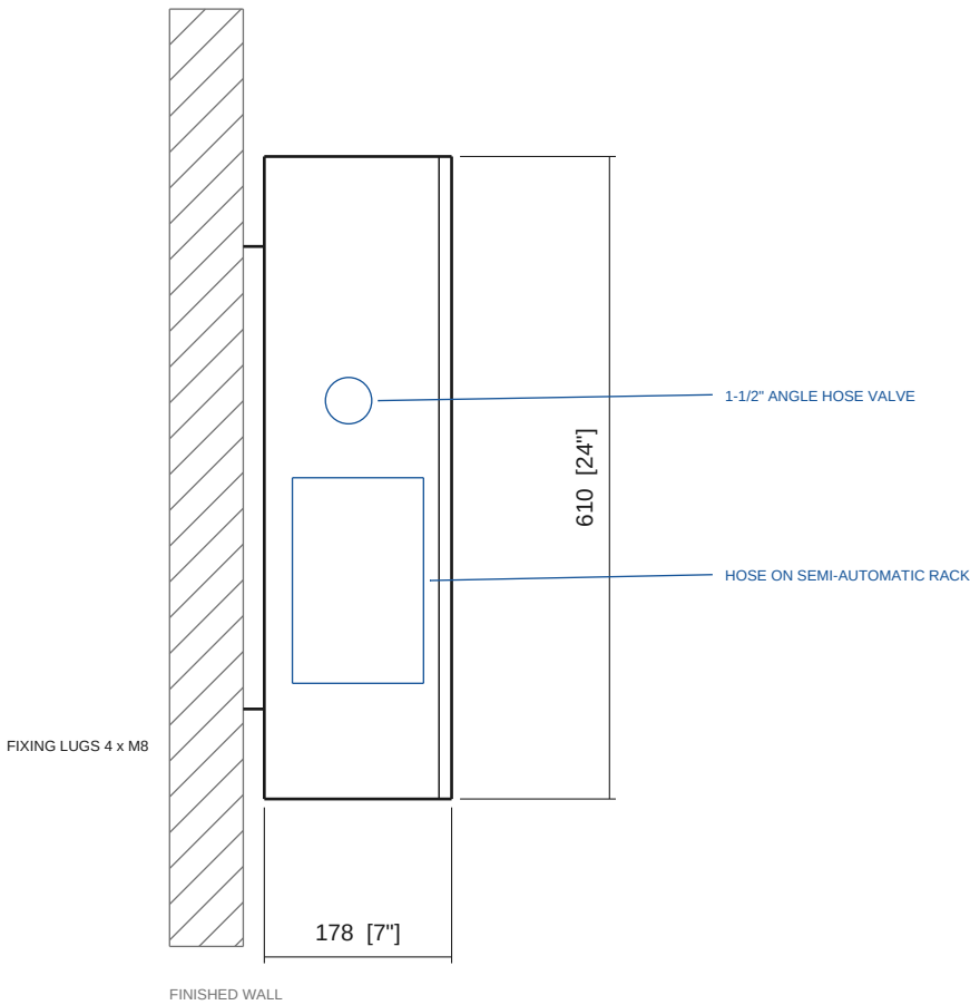
SIDE SECTION
