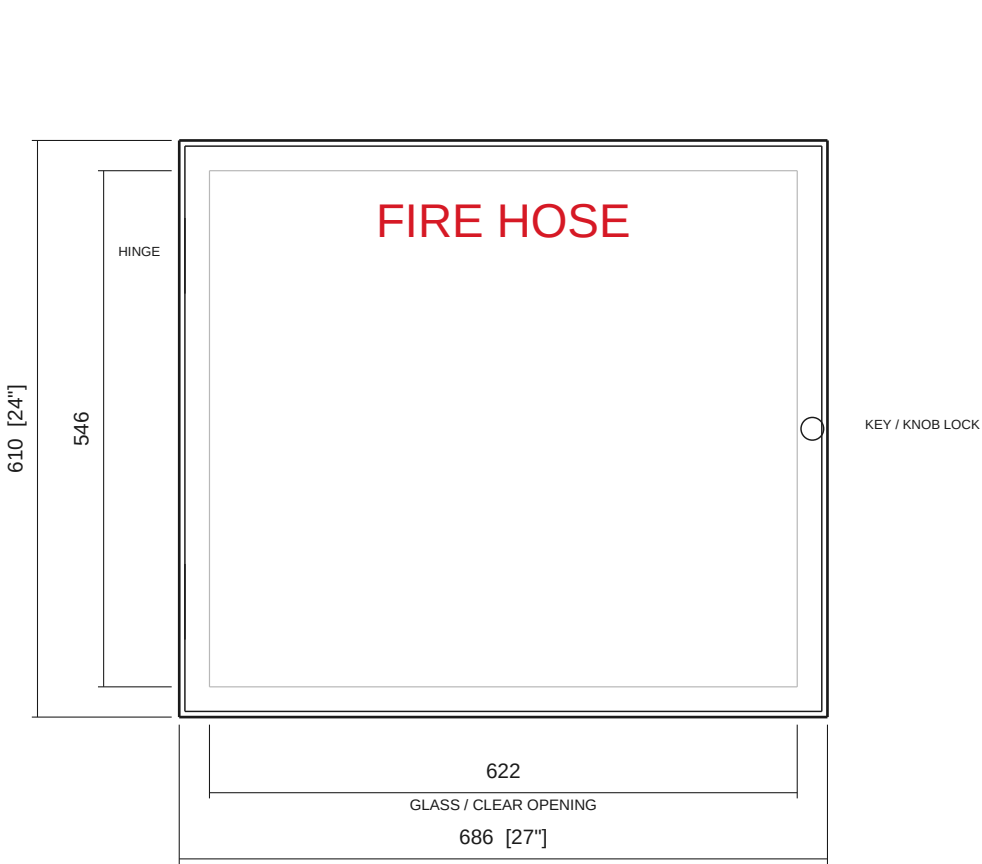
FRONT ELEVATION
